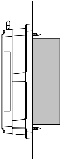
ALC22002 Recessed with Wall Cut-out Note: Recessed mount cover is for installations with the alarm mounted inside a wall cut out.
